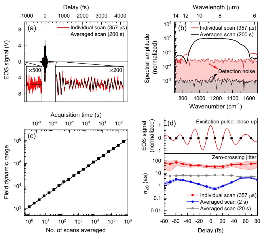
Fig. 4. Timing precision and dynamic range of delay-corrected electric field measurements. (a) Single-scan measurement of aqueous \text{DMSO}_2 solution, acquired in 357\text{ }\mu\text{s} (red) and average of 560,000 scans, which corresponds to 200 seconds of acquisition time (black). A zoom-in of a window temporally preceding the excitation pulse (left inset) shows the noise level for single (red) and averaged scans (black). The inset on the right shows the signal oscillations of the mid-IR waveform in the temporal region containing the impulsive excitation. (b) Fourier transform of the individual-scan (red solid line) and averaged-scan (black solid line) waveforms shown in (a). The shaded regions show the detection noise levels, corresponding to the individual-scan (red) and averaged-scan (black) waveforms shown in (a). (c) Spectral field amplitude dynamic range as a function of the number of scans averaged. (d) The top panel shows a close-up of the mid-IR reference waveform (red line) and the zero-crossing points (solid black circles). The standard deviation in the position of zero-crossing points ( \sigma_{zc} ) on comparing 20 consecutive individual scan (red) waveforms and averaged waveforms for averaging times of 2 s (blue) and 20 s (gray) are plotted in the bottom panel. The red and blue shaded regions show the uncertainty in the extracted timing precision, due to the detection noise (not to be confused with statistical error bars). The uncertainty corridor is not visible for the gray curve.
